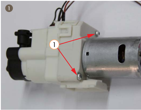
1. Take out 2 screws from dispenser valve
