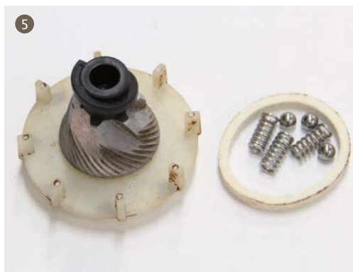
5. Take out the line pencil and conical burr group
