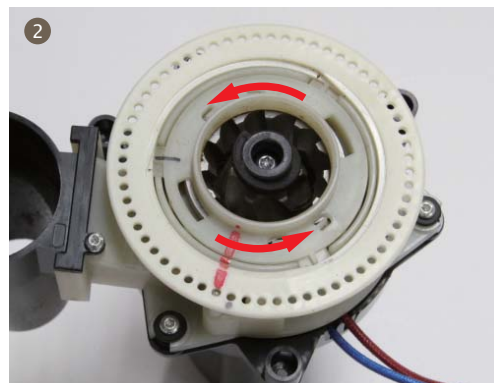
2. Rotate the upper burr group anticlockwise
