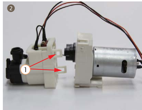
2. Loose the hook, and separate gear box for dispenser valve from the water dispenser box
