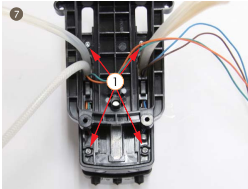
7. Disassemble 4 screws from the export group, and take out the sliding group
