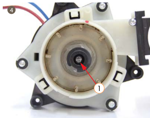
4. Disassemble 1 middle screw
