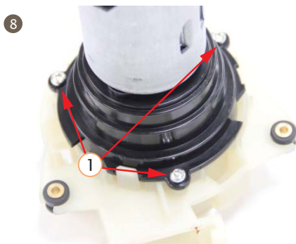
8. Install the coffee powder container into the gearbox, the bigger hook on the coffee powder container should compare to the bigger groove. Screw tightly.
