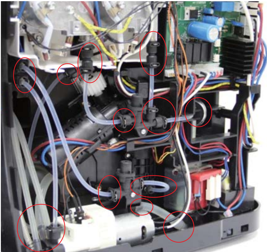
Check leakage of connectors
