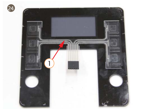
24. Take out ITO which stuck to touch screen
