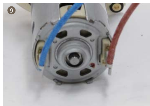
9. Install the line pencil into the grinder motor, red line correspond to the red mark.
